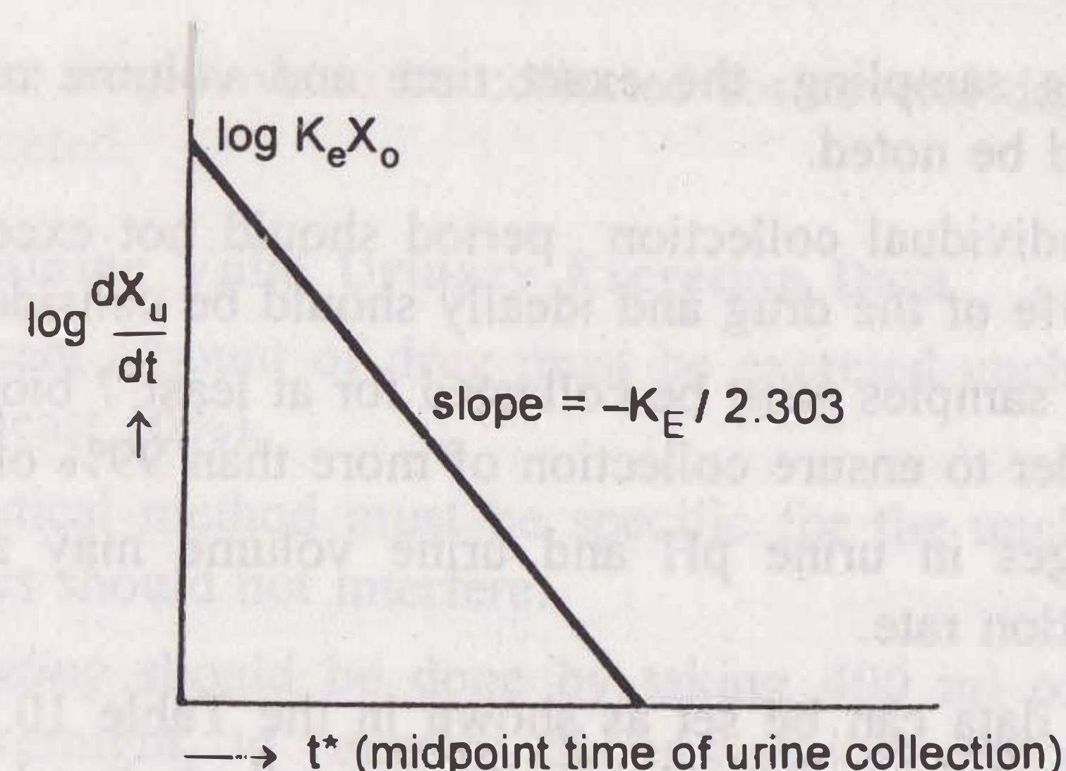
Fig. 10.10 Semilog plot of excretion rate versus midpoint time of urine collection period for computing elimination rate constant after i.v. bolus administration.
