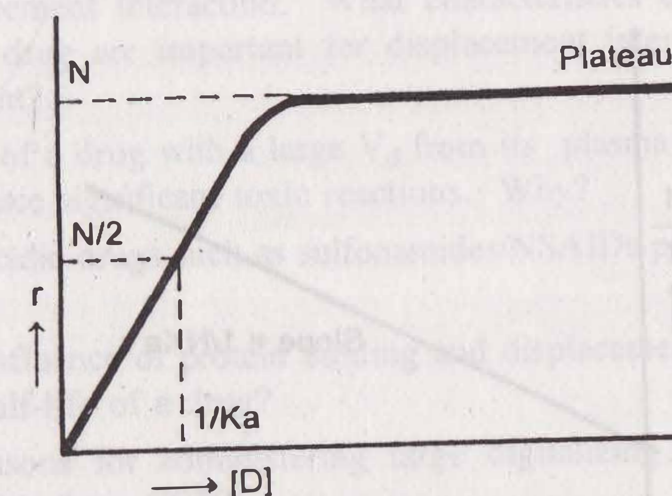
Fig. 4.4 Direct plot of r versus [D] . Note that when all the binding sites are occupied by the drug, the protein is saturated and plateau is reached. At the plateau, r = N . When r = N/2 , [D] = 1/K_a .
