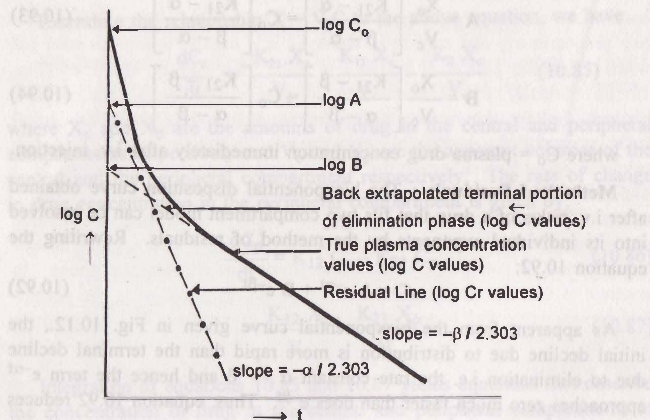
Fig. 10.13 Resolution of biexponential plasma concentration-time curve by the method of residuals for a drug that follows two-compartment kinetics on i.v. bolus administration.
