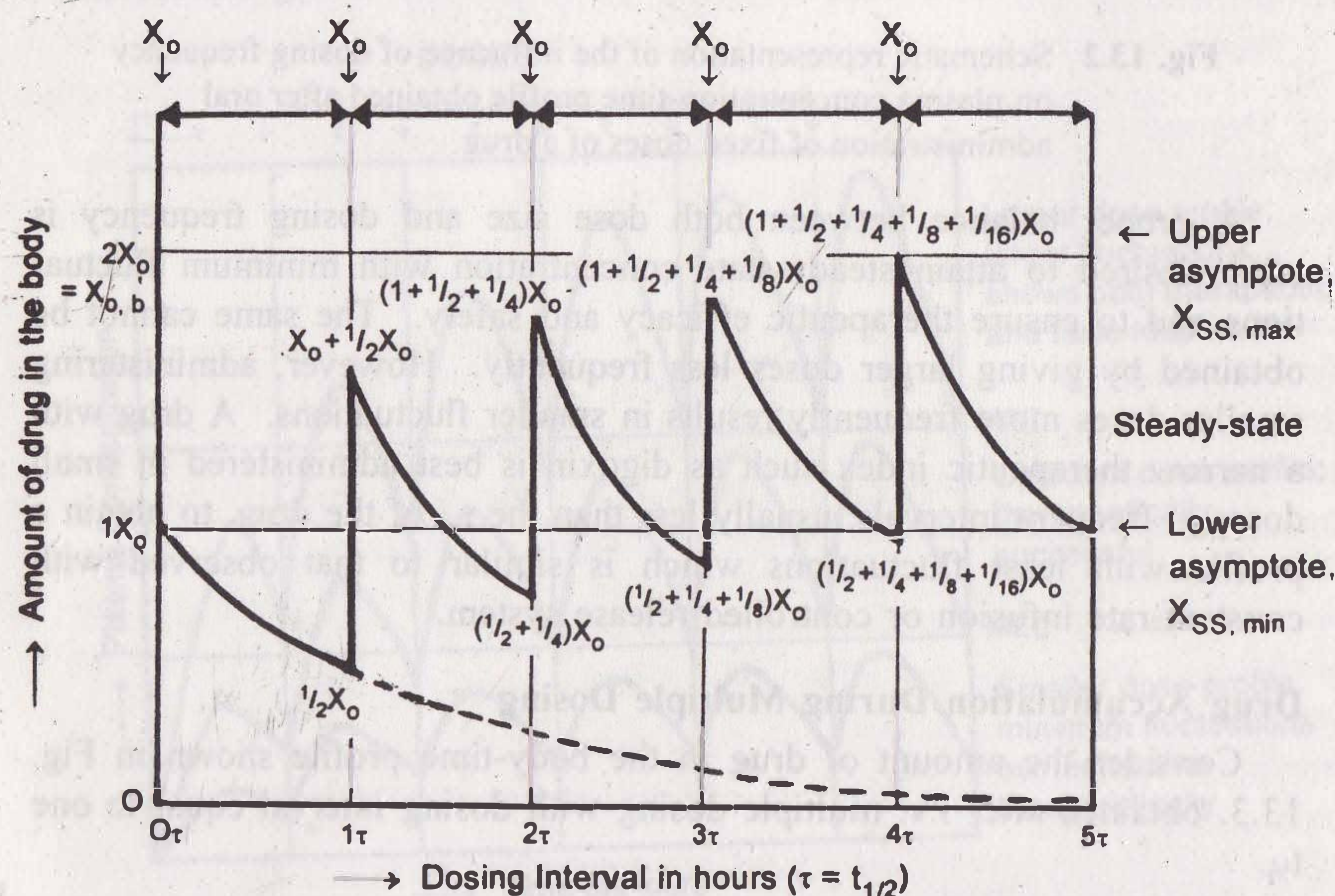
Fig.13.3 Accumulation of drug in the body during multiple dose regimen of i.v. bolus with dosing interval equal to one half-life of the drug. Approximately 5 half-lives are required for attainment of steady-state.
