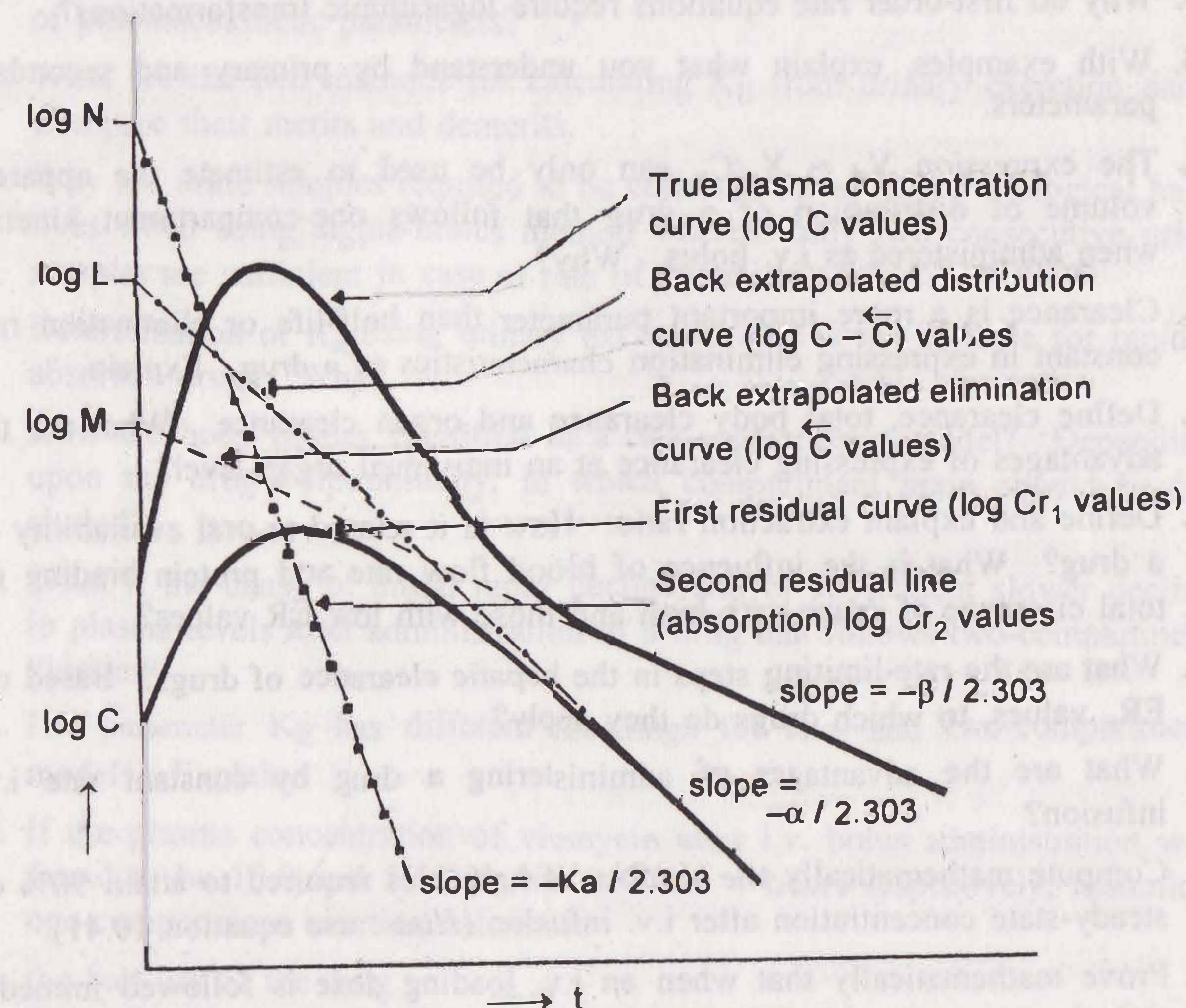
Fig. 10.14 Semilog plot of C versus t of a drug with two-compartment characteristics when administered extravascularly. The various exponents have been resolved by the method of residuals.
