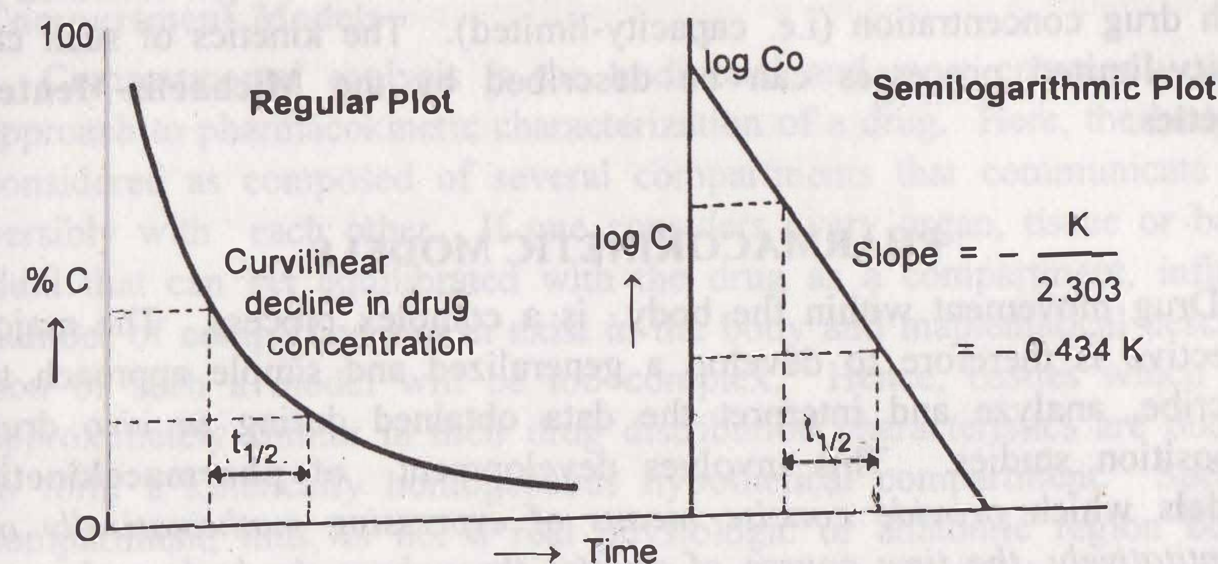
Fig. 9.4 Regular and semilog graphs of first-order kinetics
