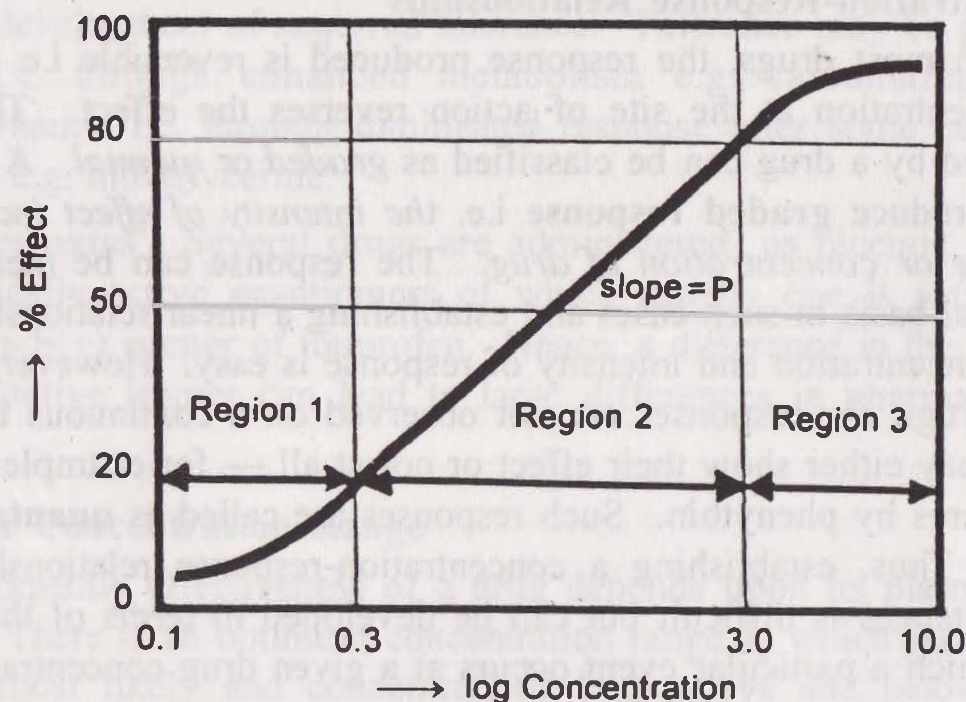
Fig. 14.1 A typical sigmoidal shape log drug concentration-effect relationship
