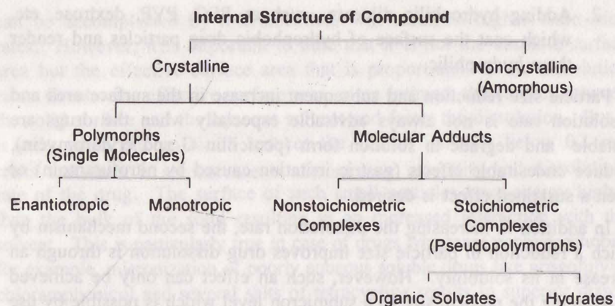
Fig. 2.14 Classification of internal structure of a compound
