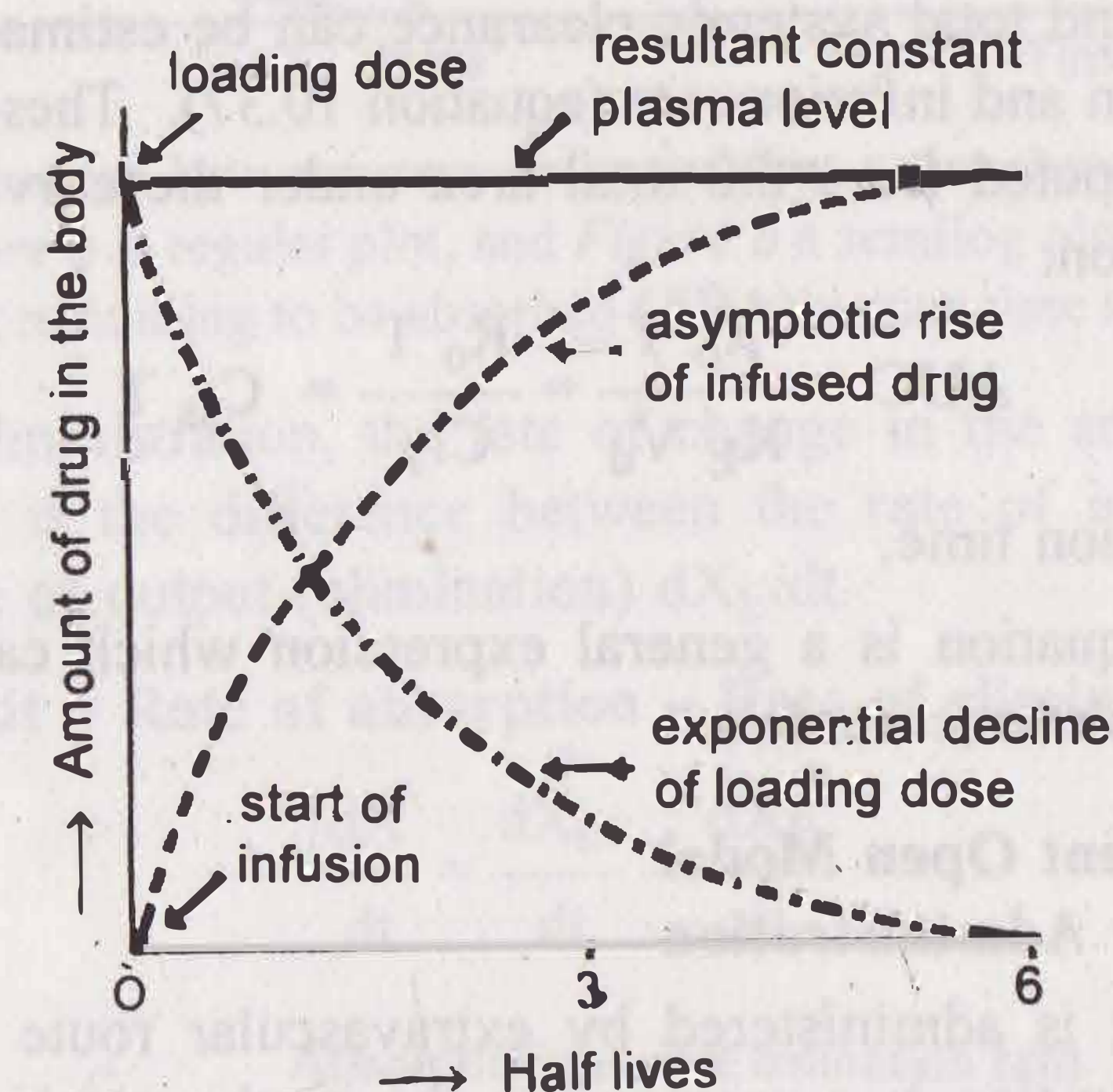
Fig. 10.5 Intravenous infusion with loading dose. As the amount of bolus dose remaining in the body falls, there is a complementary rise resulting from the infusion
